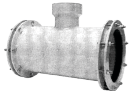
TRAVIS BOLT TITE FEMALE THREADED RISER COUPLER 18"
